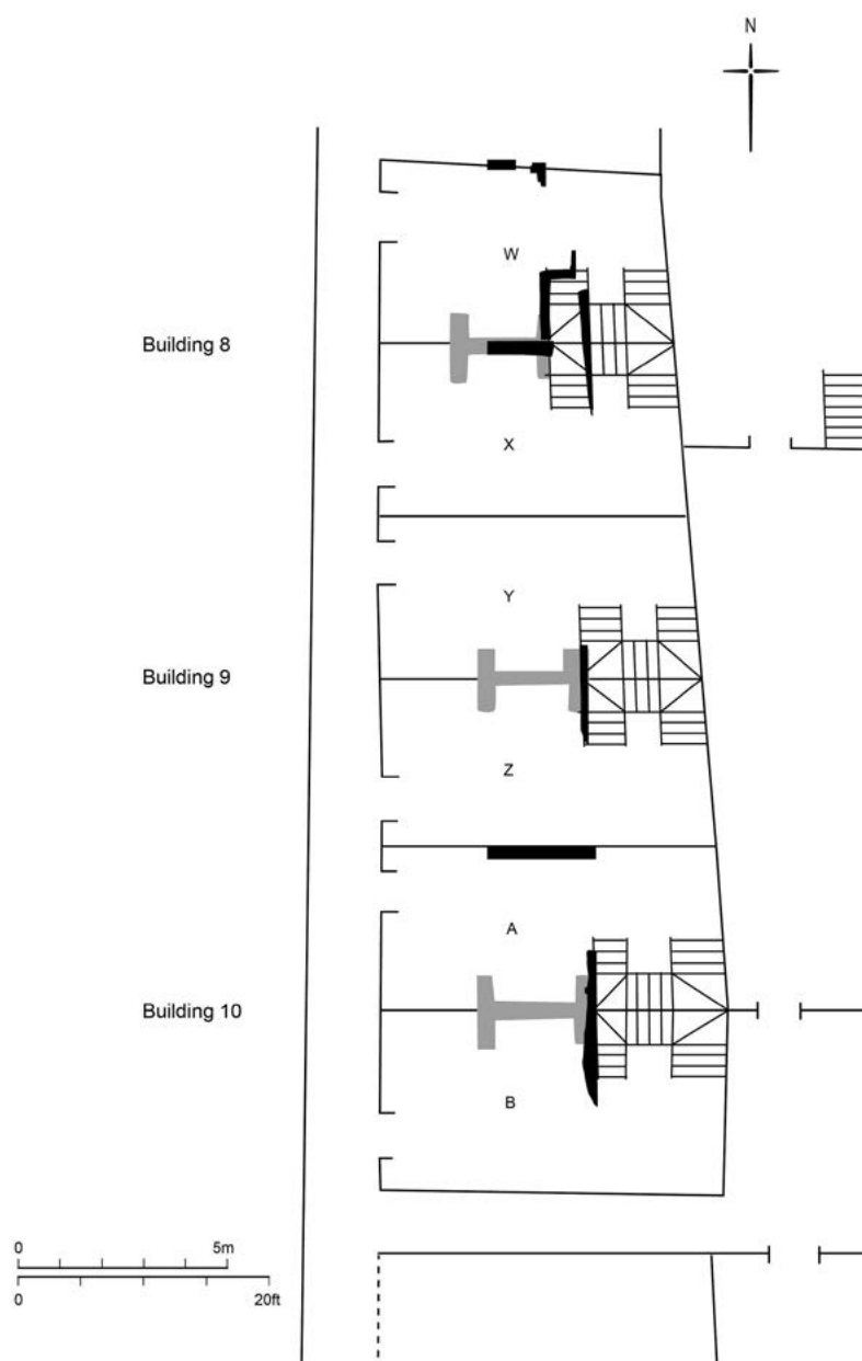
Figure 56 Seal House: the post-Fire buildings superimposed on the building outlines from the Leybourn plan of 1686 (John Schofield and Sue Cawood)
