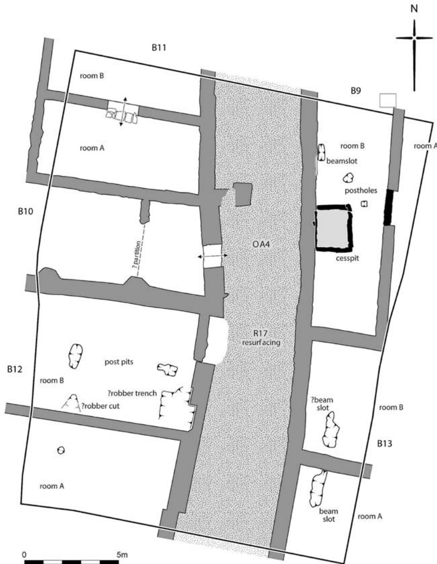
Figure 100 Billingsgate: Events 9–11, D:Buildings 9–13 (1:200)
