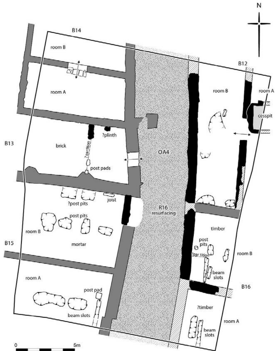
Figure 88 Billingsgate, Events 5–8: D:Buildings 9 to 13 (1:200)
