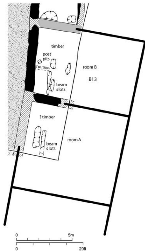
Figure 92 Billingsgate: D:Building 13 in Event 6, with property boundaries from the plan of 1680 (1:200)
