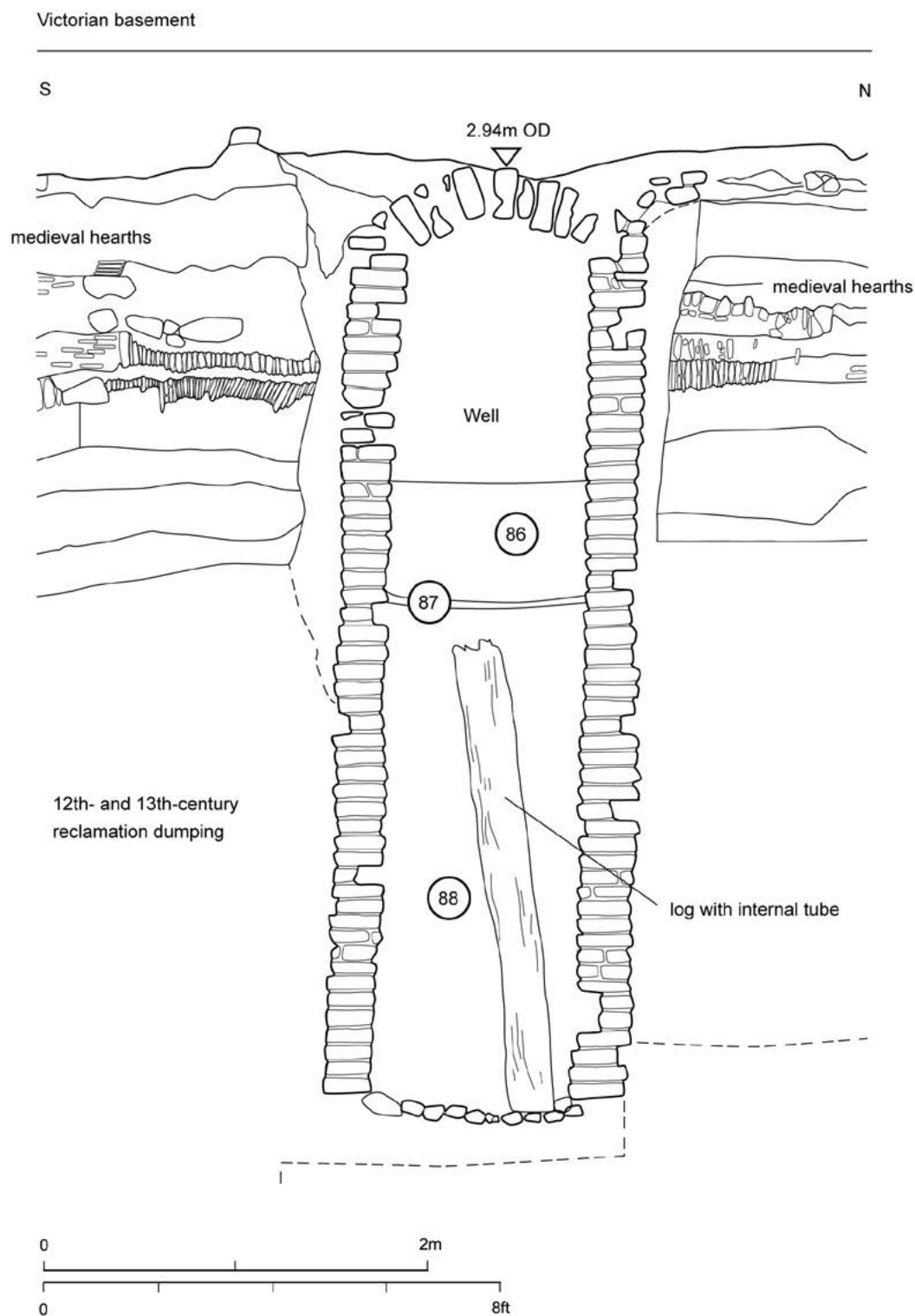
Figure 44 Seal House: extract from the section along the south part of the west baulk, showing well B[26] and within it a log with an internal longitudinal bored cavity, a rising main for a pump. The well was dug through the remains of medieval buildings (compare Figure 43) and 12th- and 13th-century reclamation dumping beneath (the edge of the medieval waterfront was about 4m to the south, to the left) (Sue Cawood)
