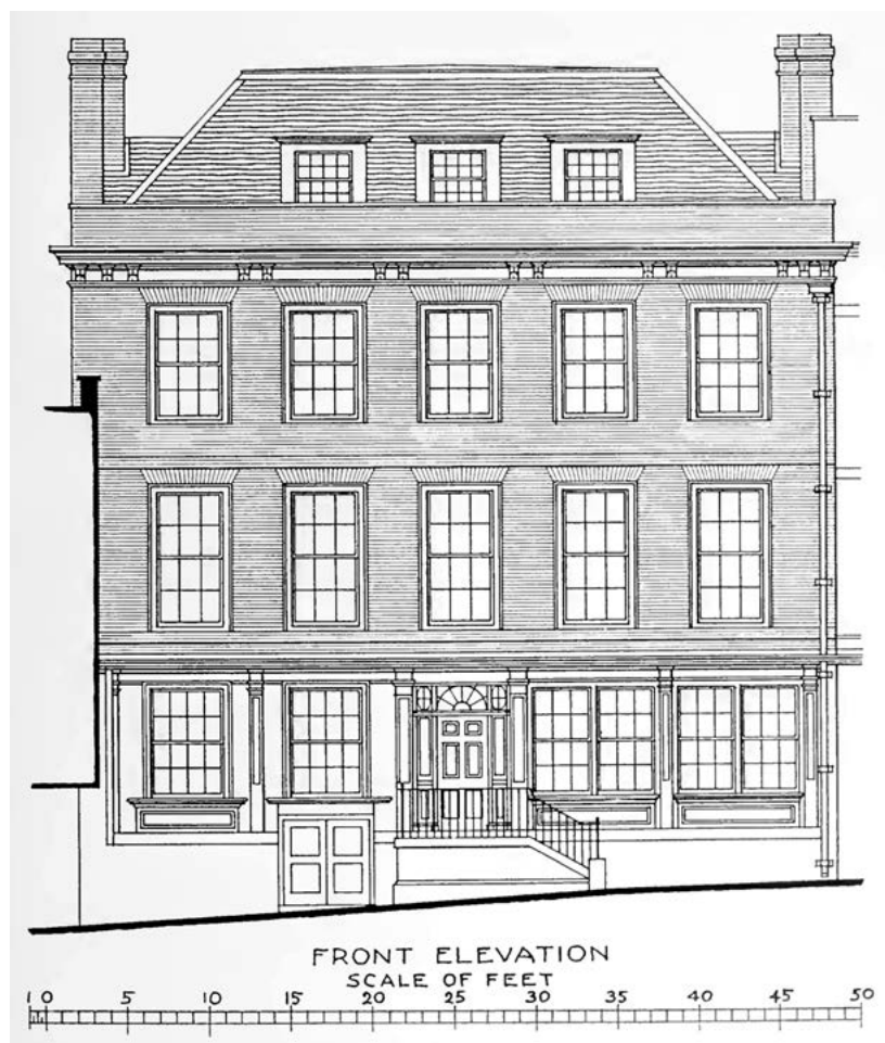
Figure 146 The north (front) elevation of 34 Great Tower Street in 1934 (SoL 15, pl 42; drawn by A E Gurney). Originally the generous windows would have been of the transom form, like those at Fishmongers' Hall (Figure 58), and probably of timber; here they have been replaced
