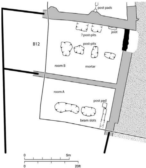
Figure 96 Billingsgate: D:Building 12, as amended in Event 8, with property boundaries from the plan of 1680 (1:200)
