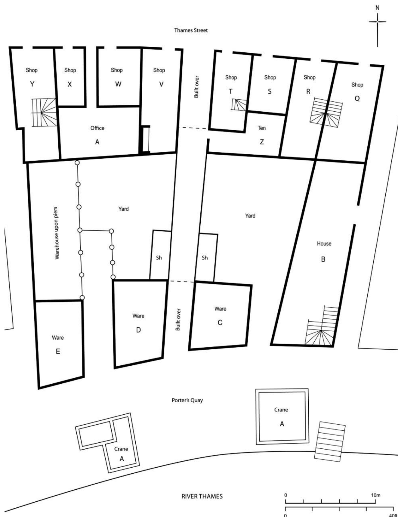
Figure 149 Porter's Quay, Thames Street, in 1686 (William Leybourn, Fishmongers' Plan Book , f3; redrawn by Sue Cawood). The initial letters indicate tenancies; Ware=Warehouse. The eight tenements at the front, Tenement Z and the Office A had four floors and cellars; Warehouses C, D and E had vaults beneath
