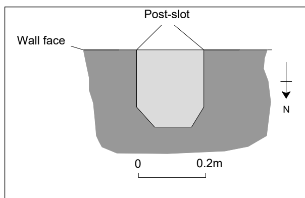
Figure 2.26. Fenton Hill: plan view of post-slot 114, showing chamfered corners
