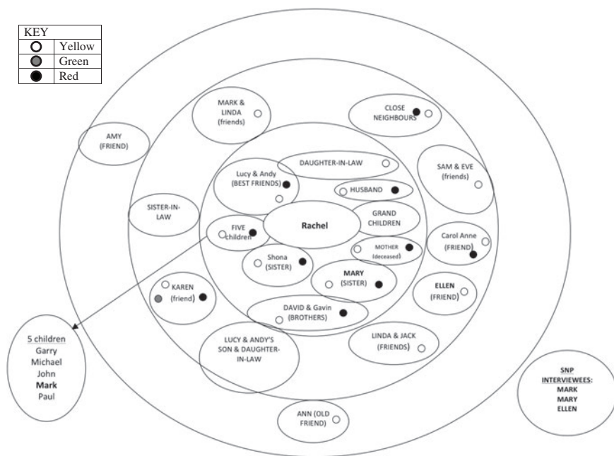
Figure 2.1 Social networks.
