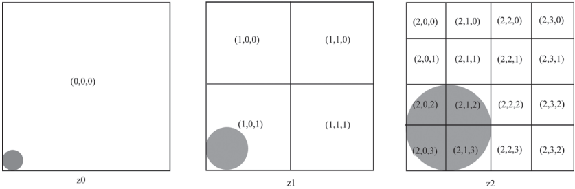
Figure 7.3. Zoom and the z-axis. Mapbox tile layer coordinates (z, x, y) at three zoom levels z_0 and z_2 , showing the relative size of a symbolic object.
