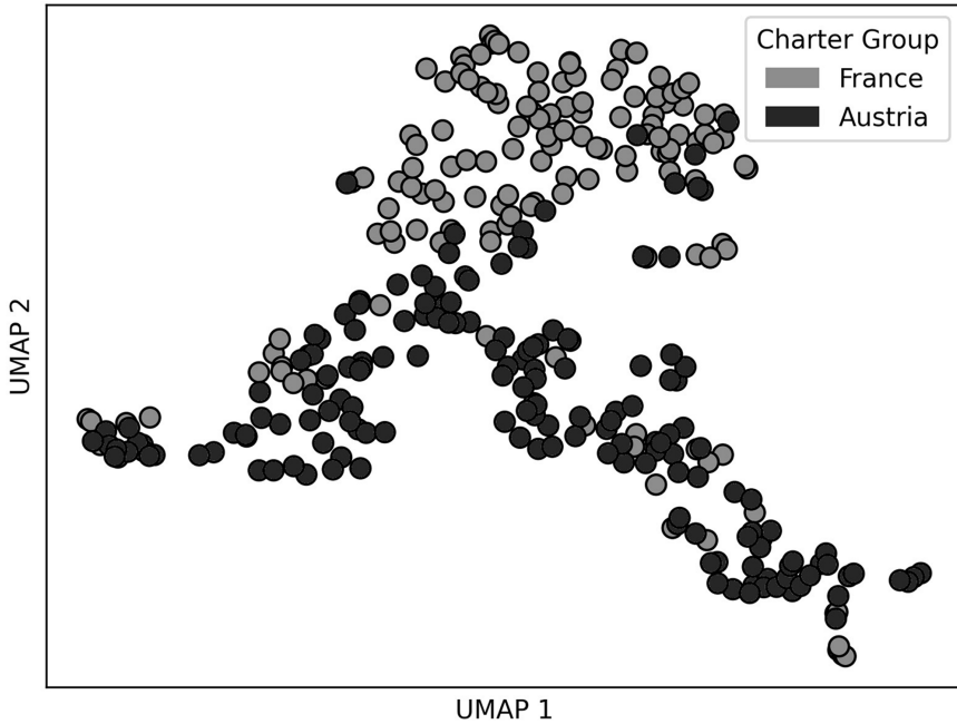
Fig. 6: Binarized charters with large HOG feature extraction
