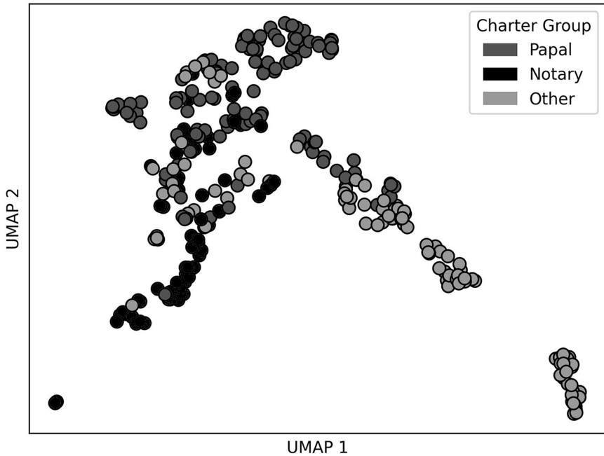
Fig. 8: Charters with CLAHE & Retinex preprocessing and large HOG feature extraction
