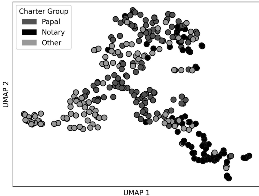
Fig. 5: Binarized charters with large HOG feature extraction (i. e. 64 x 64 cell size, 128 x 128 block size)
