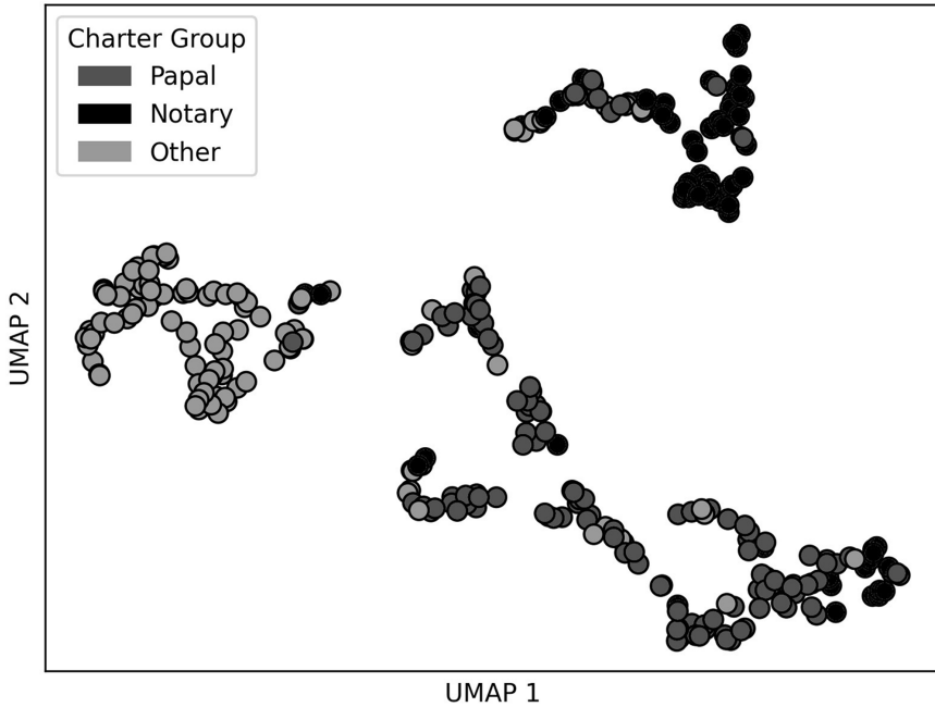
Fig. 4: Binarized charters with CNN feature extraction
